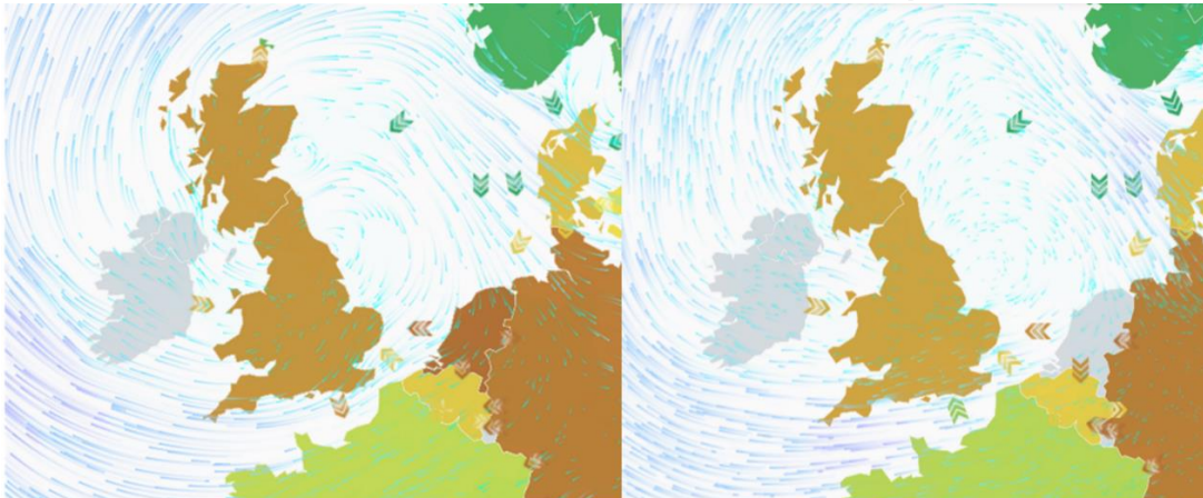
Wind conditions 7 am, 17 December 2021
